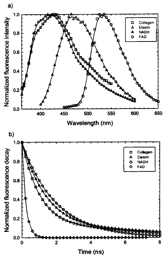
FIG. 9. Fluorescence emission spectra and decay traces of elastin (420 nm), collagens type I from calfskin (410 nm), NADH (450 nm), and FAD (550 nm): (a) time-integrated spectra; (b) deconvoluted (based on the Laguerre basis expansion technique) fluorescence decay traces obtained at the specified wavelength.
